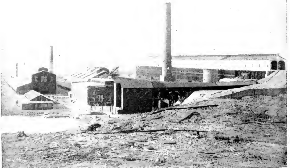
Fig. 69—General View of Blast Furnace and Converter Departments, Copper Cliff.
